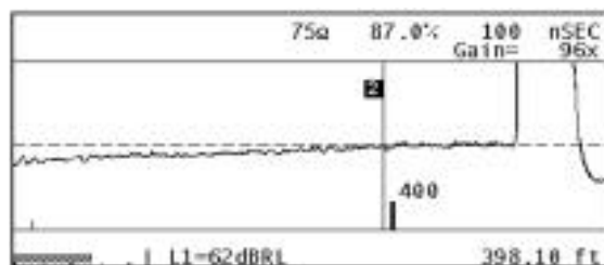
Typical TDR test misses the fault completely.
