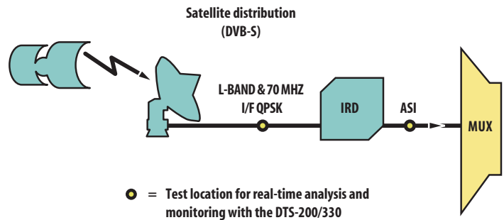
MPEG over Satellite verification at all points of a Satellite network
